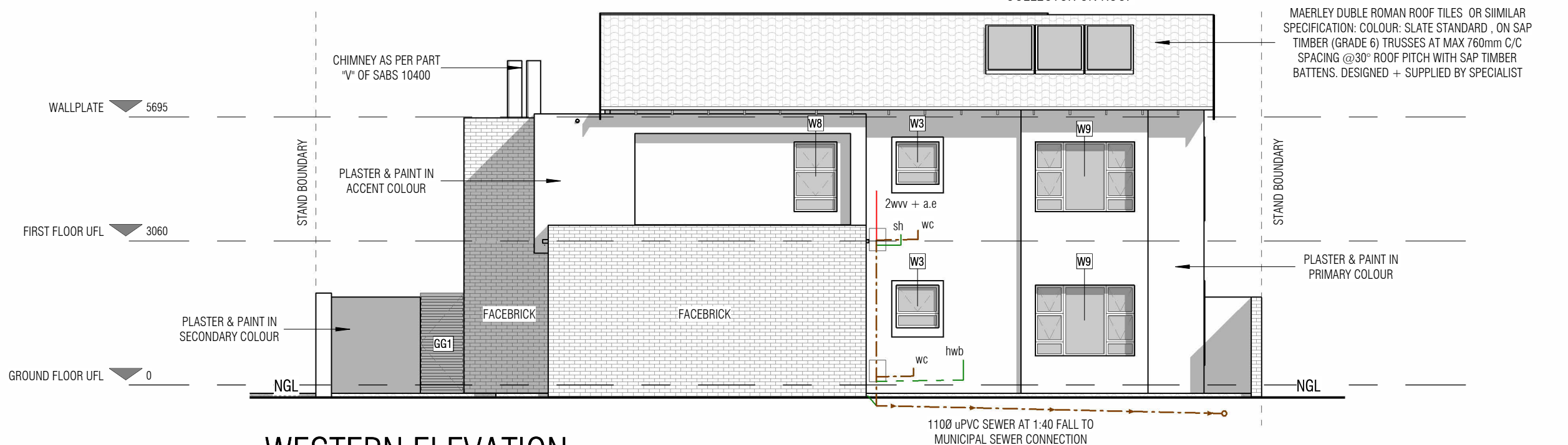
4 WESTERN ELEVATION 1 : 100
