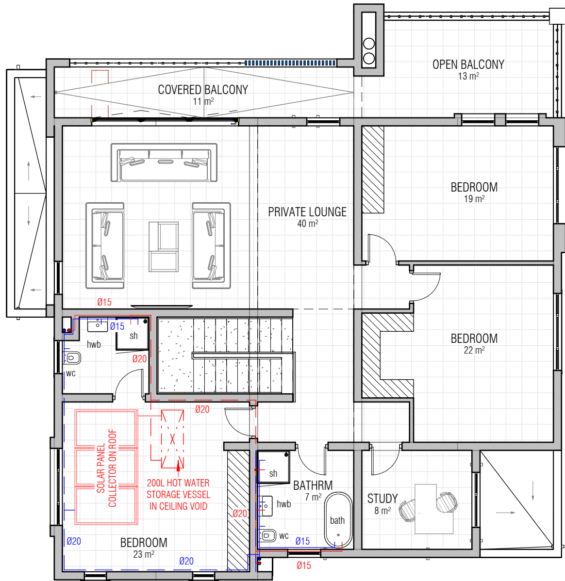
2 FF - WATER RETICULATION LAYOUT 1 : 100
