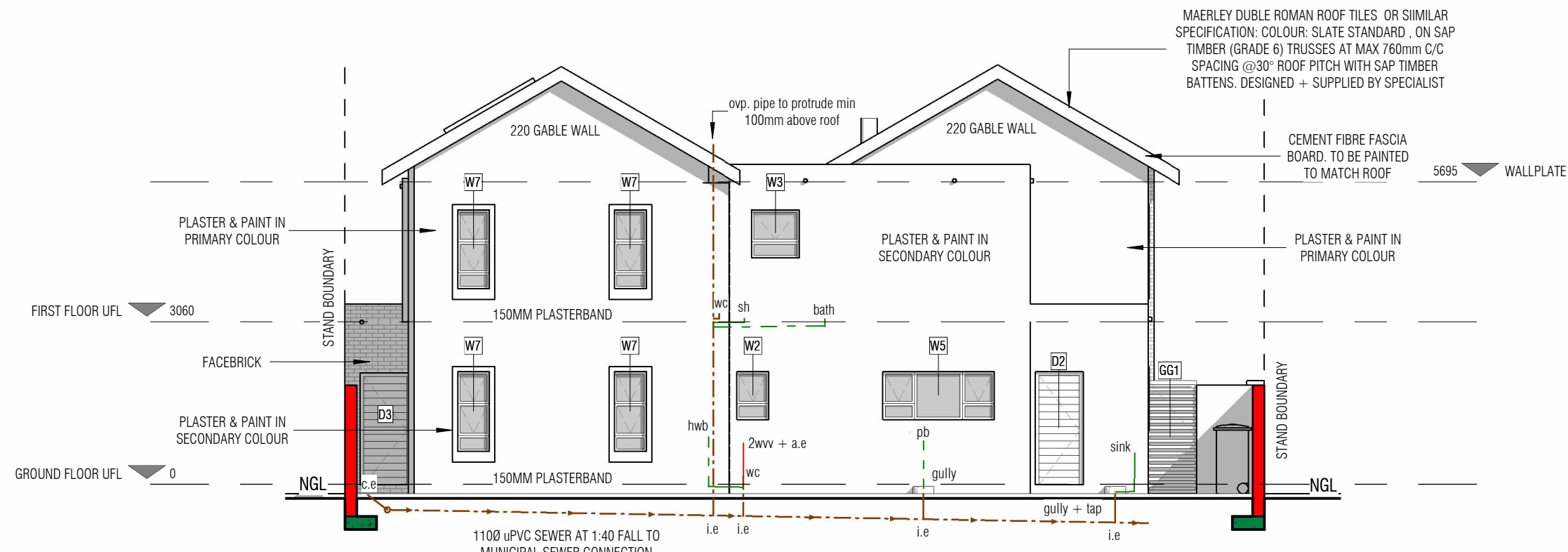
3 SOUTHERN ELEVATION 1 : 100
