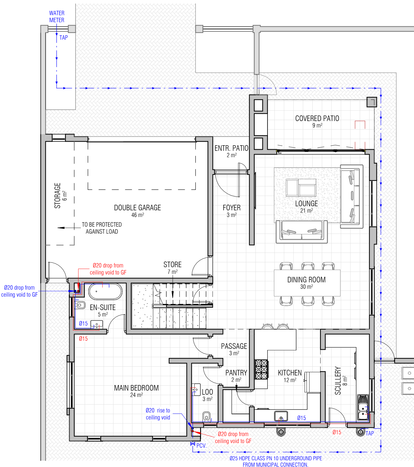
1 GF - WATER RETICULATION LAYOUT 1 : 100
