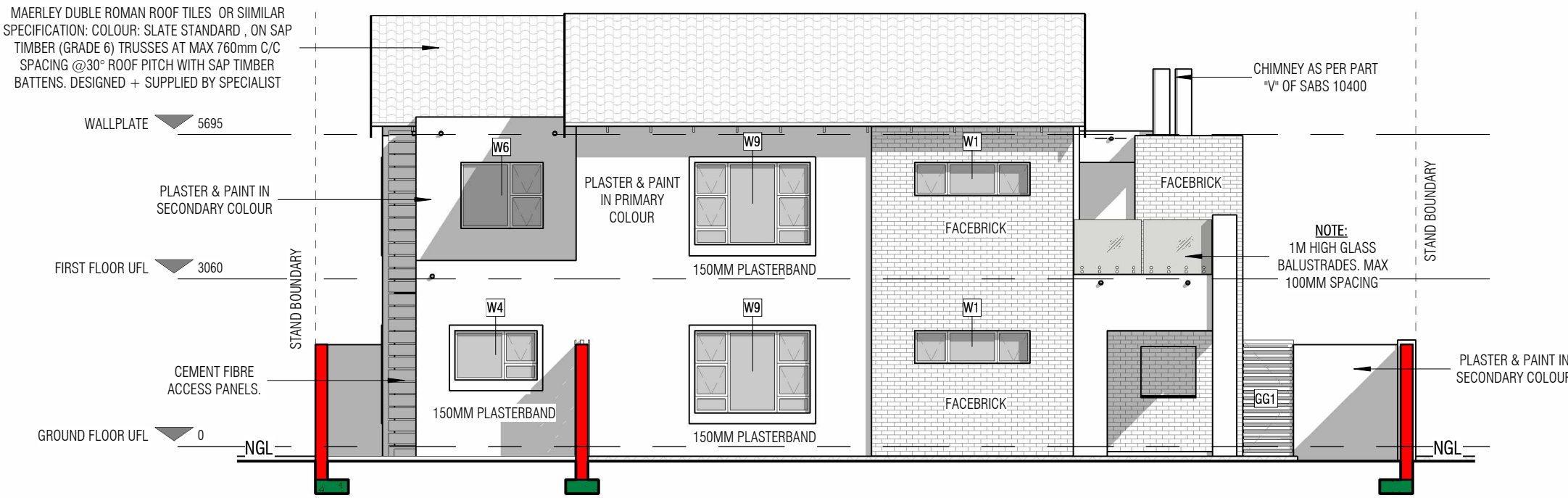
2 EASTERN ELEVATION 1 : 100
